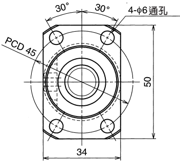
俯視X-X
