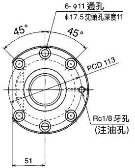
俯視 X-X
